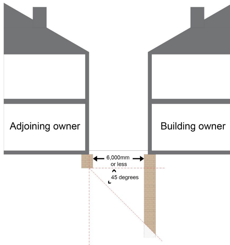
Figure 10: Section 6(2) excavations
