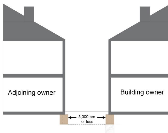
Figure 9: Section 6(1) excavations
